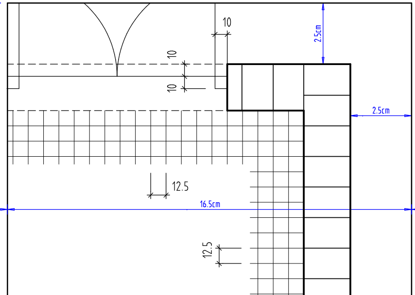
GRUNDRISS M 1:20 [cm]
