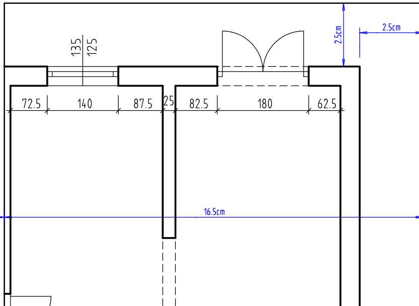
GRUNDRISS M 1:50 [cm]
